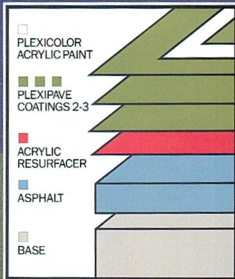
Plexipave® System over Asphalt Base
