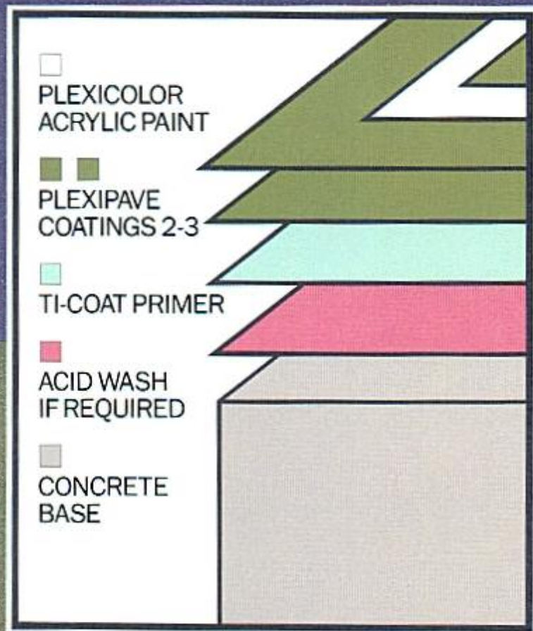
Plexipave® System over Concrete Base
